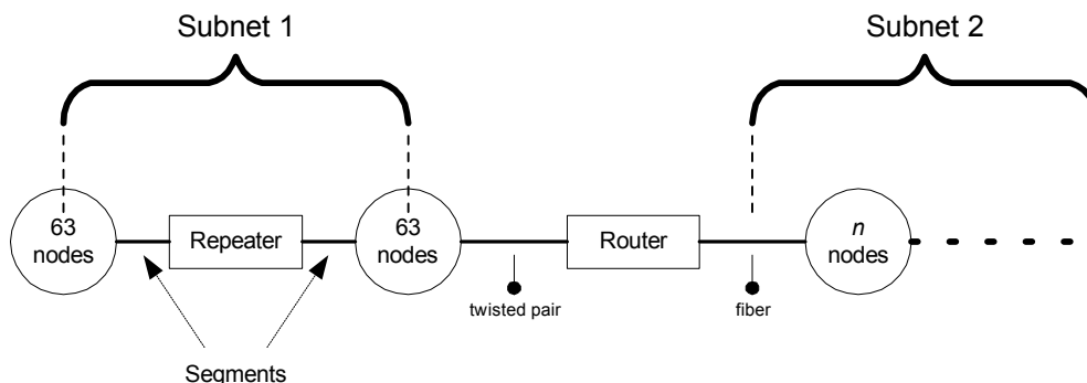
Figure 2. Network Topology.
